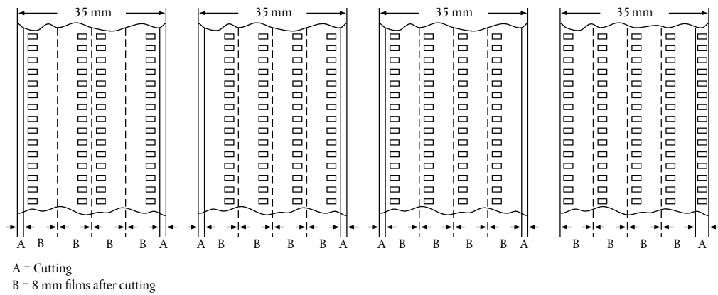
Examples of films with several image bands
