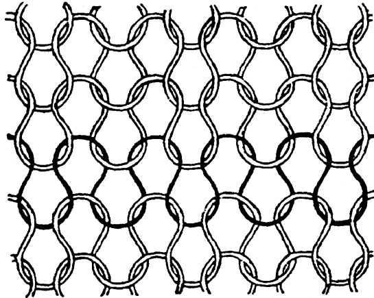
Figure 4 Ribbed 1 plain × 1 purl
